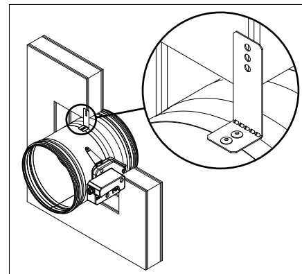
Fix the damper to the wall using screws (screw hole is 6mm in diameter)
