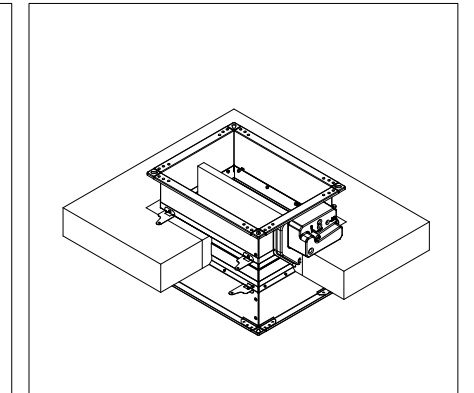
Fill the space between the damper and the slab with mortar
