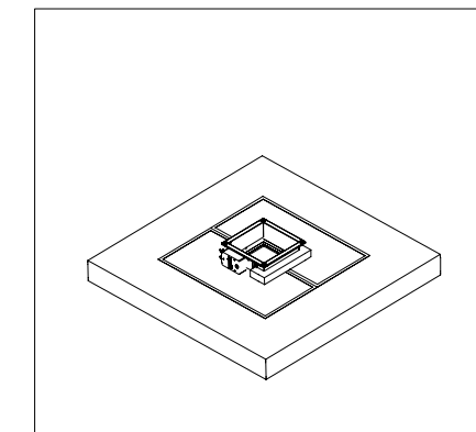
Connections of mineral wool must be sealed with intumescent fire resistant sealant. Mineral wool and damper casing must be coated with 2 mm thick fire protection coating
