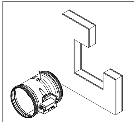
Place the damper in an opening according to table (on pg. 366)
