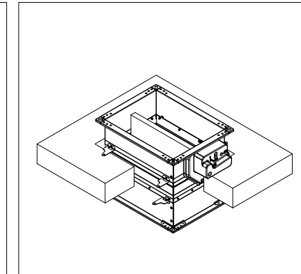
Fix the damper to the slab using screws
