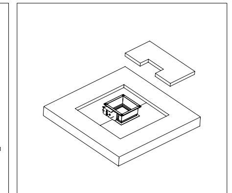
Space between casing and ceiling must be closed with two layers of mineral wool (density 140 kg/m 3 or more, 50 mm thick, coated on one side)
