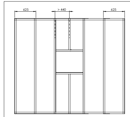
Realization of the steel construction
