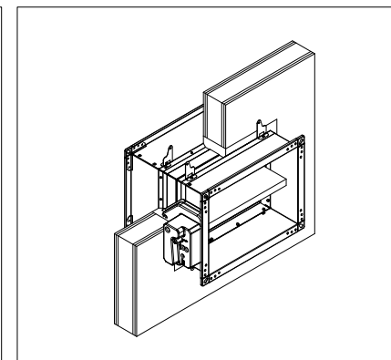
Fill the space between the damper and the wall with mineral wool
