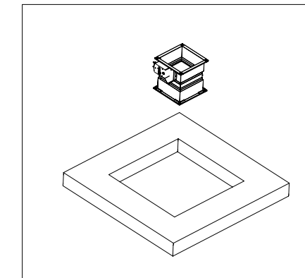
Recommended ceiling opening for fire damper installation is B(H) + 400mm, but openings from B(H) + 80...600 mm can also be used
