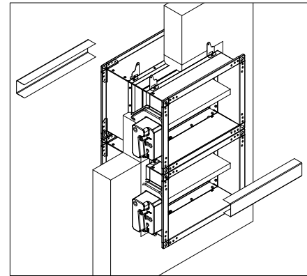
Place the installation kit to the dampers
